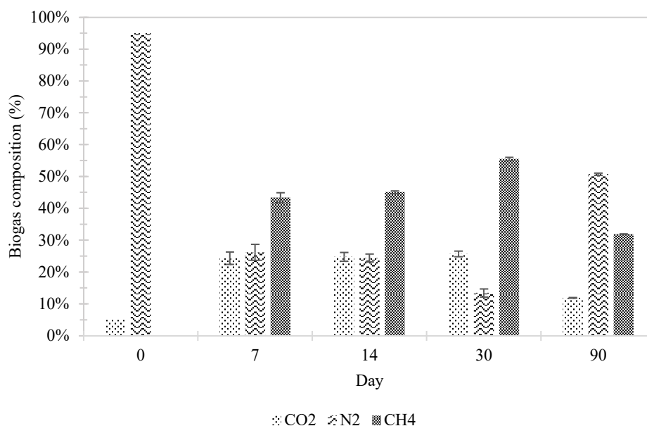
Figure 3. Biogas composition throughout the experiment
