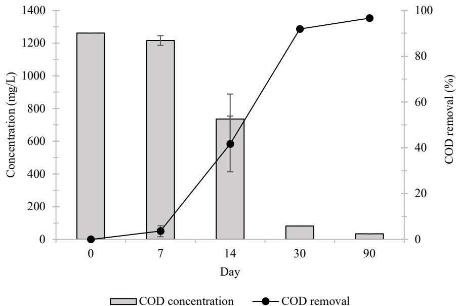
Figure 2. COD removal performance throughout experiment
