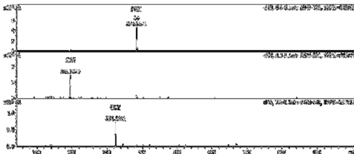
Figure 4. Mass spectrometry of PRZ (5.9 min), CAF (6.2 min) and GLZ (8.0 min)
