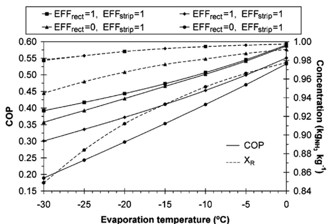
Fig. 24 Variation of COP versus the evaporation temperature in the presence of distillation column (Reprinted from Fernández-Seara and Sieres [142], with permission from publisher).
