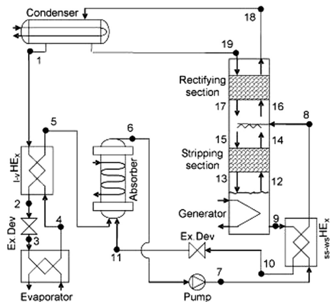
Fig. 23 Schematic diagram of the absorption system and distillation column (Reprinted from Fernández-Seara and Sieres [142], with permission from publisher).
