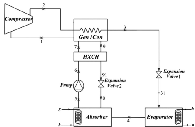
Fig. 27 A schematic diagram of the hybrid single-effect absorption/vapour recompression cycle (Reprinted from Razmi et al. [170], with permission from publisher).
