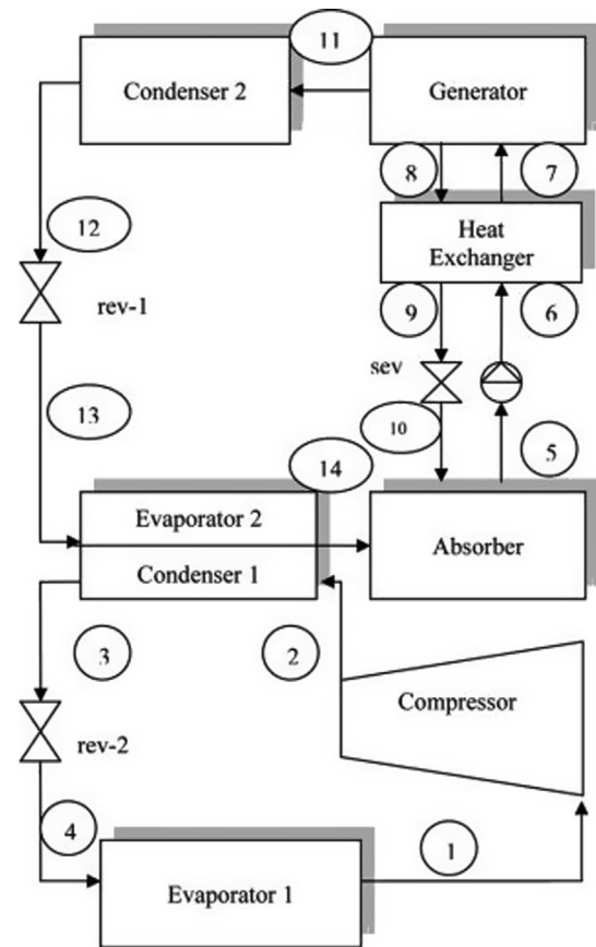
Fig. 26 Schematic of single effect compression-absorption cascade refrigeration cycle (Reprinted from Wang et al. [165], with permission from publisher).
