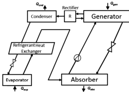
Fig. 11 A schematic diagram of simple GAX cycle.
